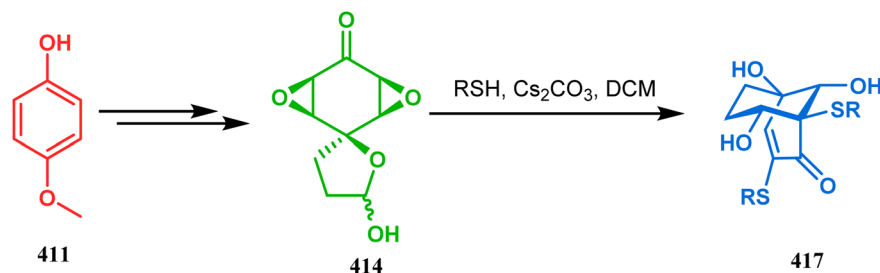
Scheme 94 Synthesis of bicyclo[3.3.1]non3-en-2-one system from spiropdiepoxyketone obtained from 411 through three-membered ring-opening and rearrangement reaction.
